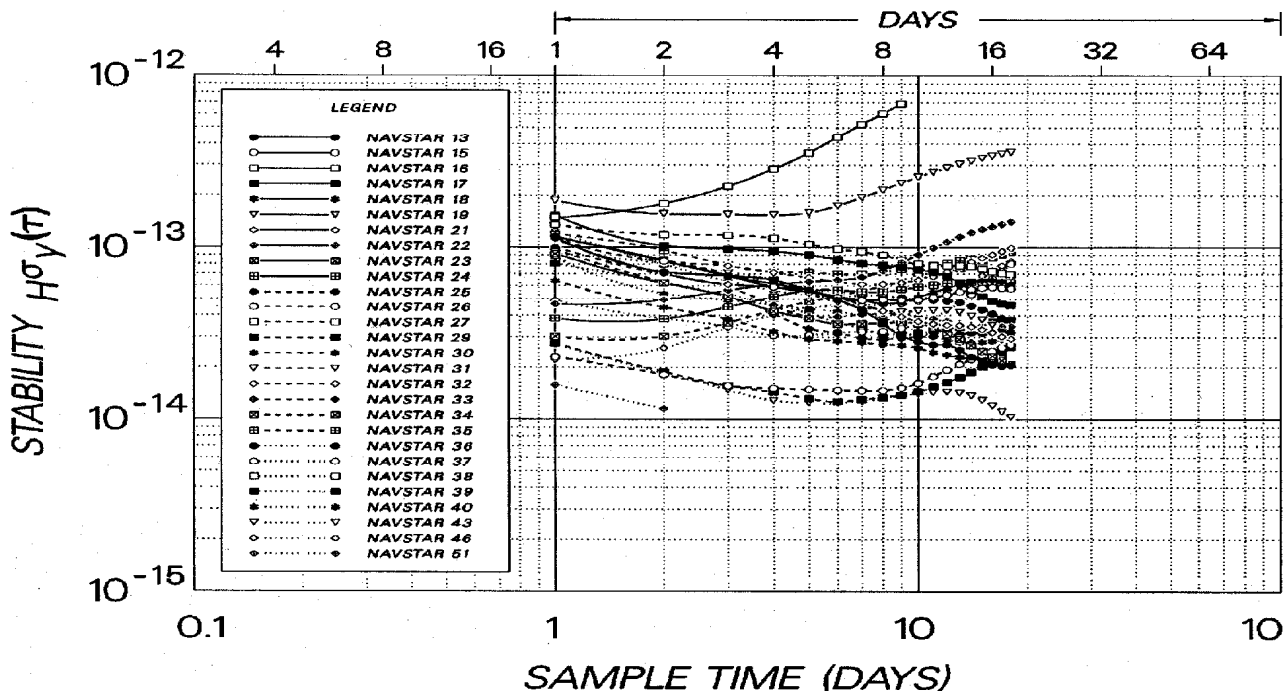
Figure 2: Hadamard-deviation frequency stability of individual GPS satellite clocks vs. USNO Master Clock for the period 1 January to 1 July, 2000 [18].
