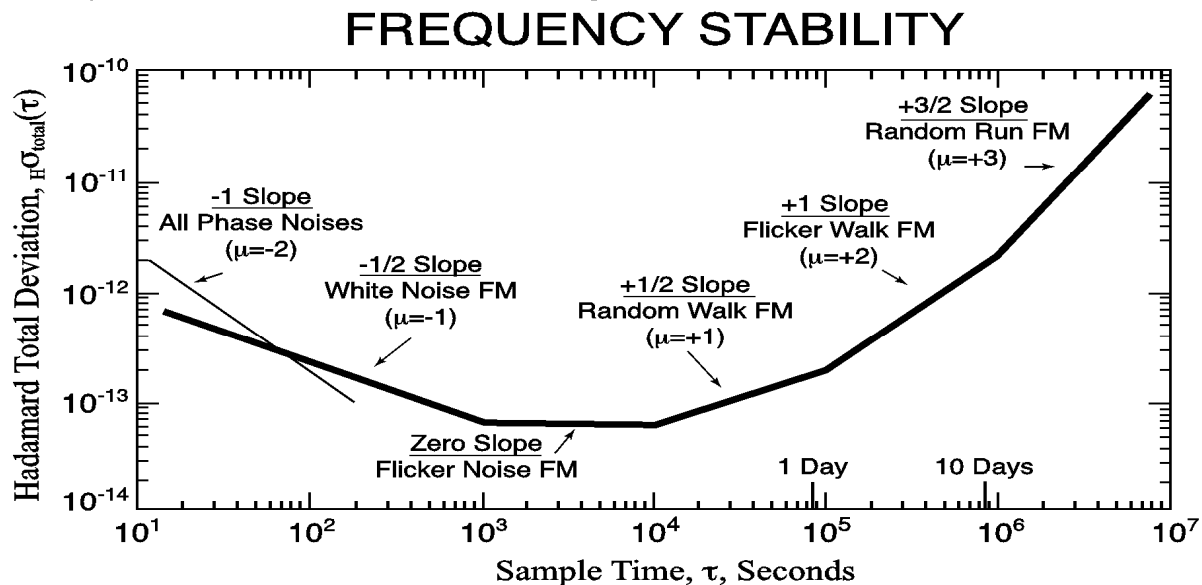
Figure 1: The Hadamard deviation (root Hvar) shows FM power-law noises as straight lines in addition to PM sources of noise for \tau -domain power-law exponent \mu (that is, {}_{\text{H}}\sigma_y^2(\tau) \propto \tau^\mu ) range of -2 \leq \mu \leq 3 . We define a new estimator that can be interpreted identically called Hadamard-total deviation (root TotHvar) and that has significantly improved confidence at long term. The Hadamard-total deviation is insensitive to linear frequency drift that can mask characteristic random noise typically encountered here in the region where \tau = one-week and longer. The goal is to identify \mu even-integer power-law noises and accurately estimate their levels in order to set system parameters associated with the GPS Kalman filter.
